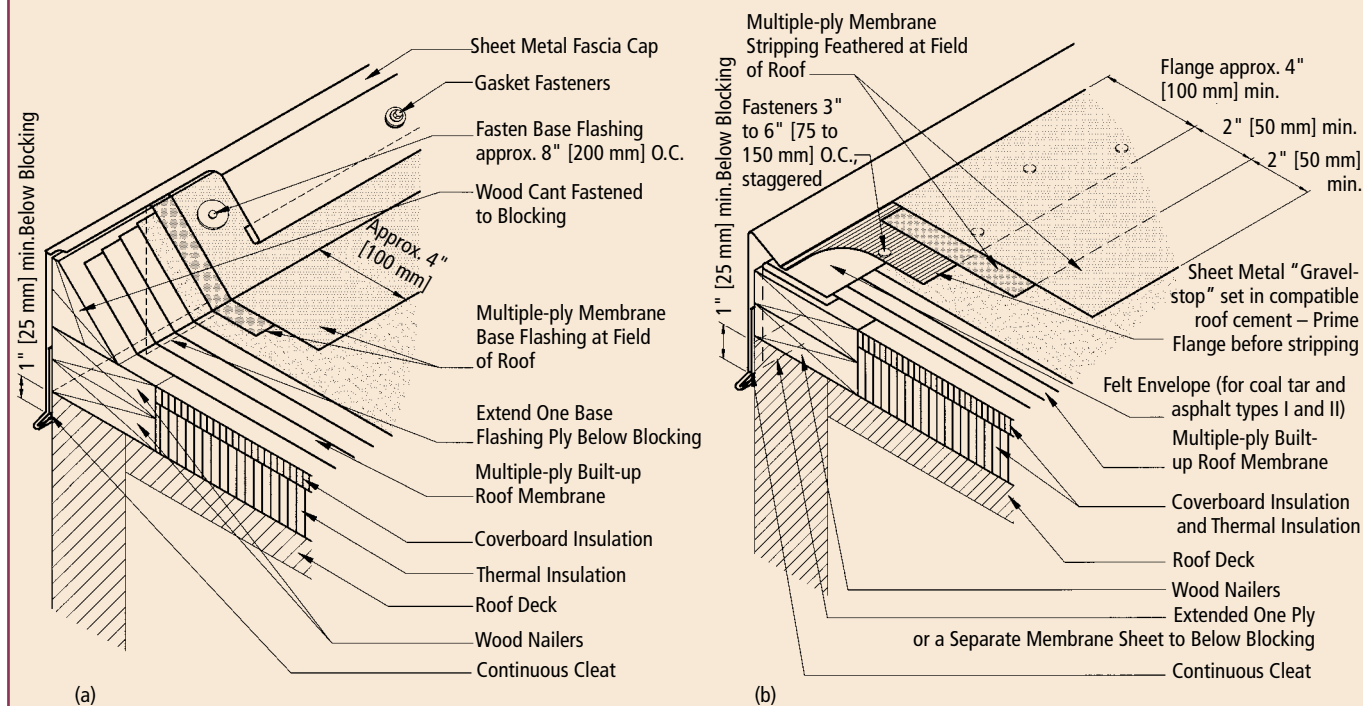
Fig. 5.8.3(a) &amp; (b) Low parapet details.
