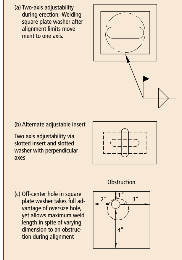
Fig. 4.5.14 Slotted or oversize holes.
