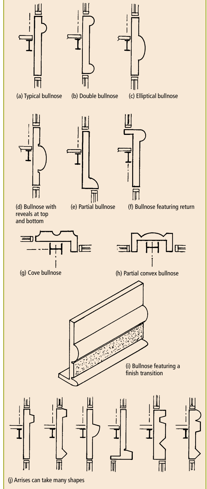
Fig. 3.3.25 Bullnoses and Arrises.
