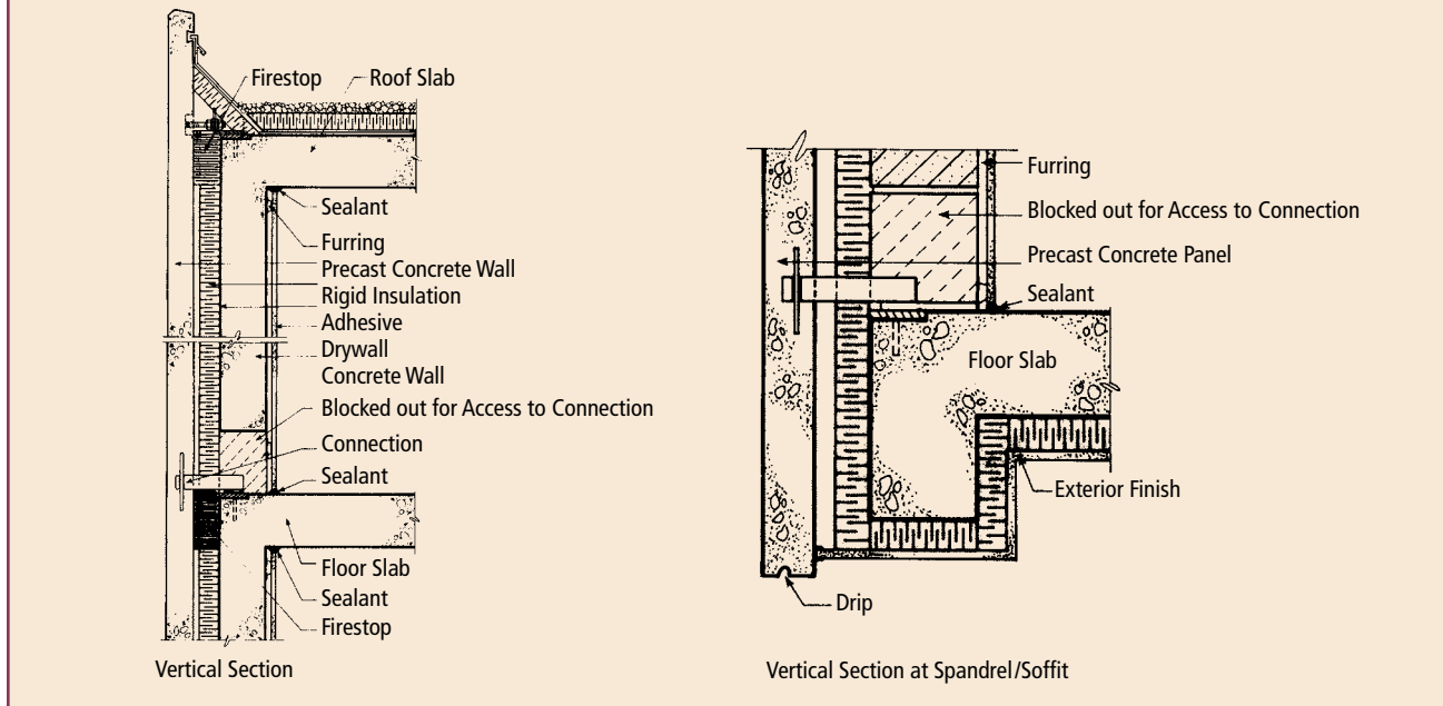
Fig. 5.3.36 Cladding erected over previously erected wall.
