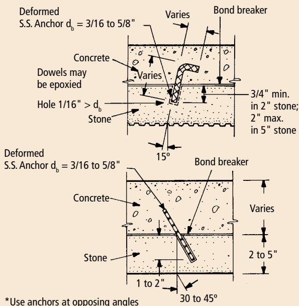
Fig. 3.5.84 Typical anchors for limestone veneer.
