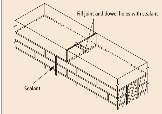
Fig. 3.5.105 Coping joints.
