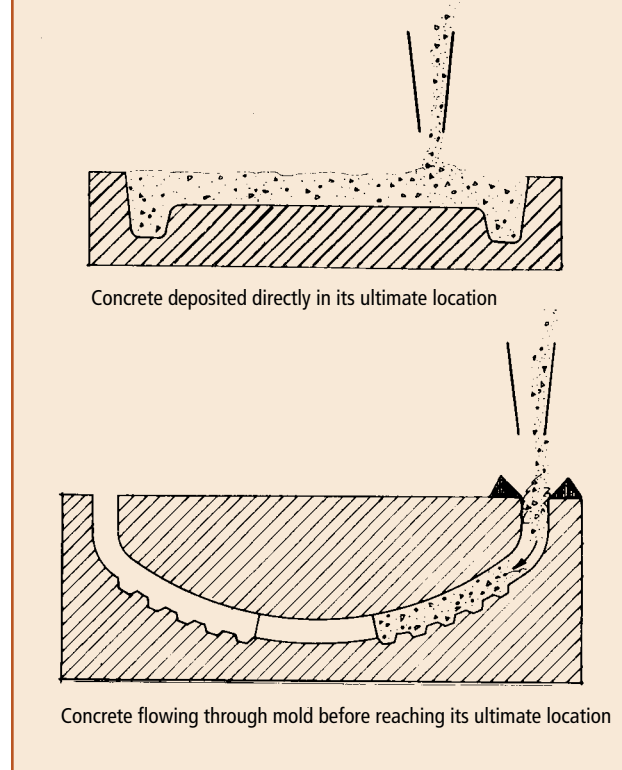
Fig. 3.2.8 Different concrete placing conditions.
