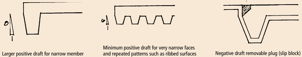
Fig. 3.3.4 Draft requirements.
