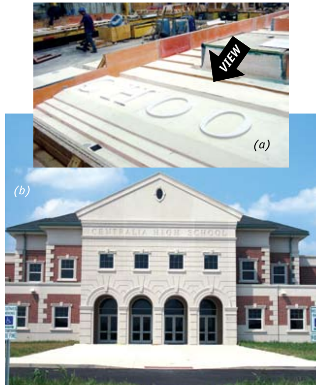
Fig. 3.5.21(a) & (b) Letters are reversed in the mold. Note the letter “c” that is part of the word “school”. Centralia High School, Centralia, Illinois; Architect: FGM Architects Engineers, Inc.; Photos: (a) Jim Lewis, (b) Max Rogers.
