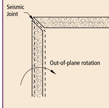
Fig. 4.5.5 Corner joint made wider to avoid collision.
