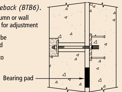
Fig. 4.5.43 Bolted tieback (BTB7).
