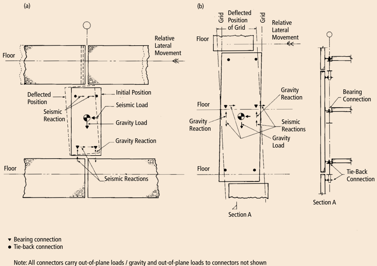
Fig. 4.5.9 Tieback or push-pull connection for a tall precast spandrel attached to a steel beam. Bearing connection at top, tieback connection at bottom. Illustration: Chris Arnold / Tony Alexander, WBDG Building Envelope Study, National Institute of Building Sciences, Washington, DC.
