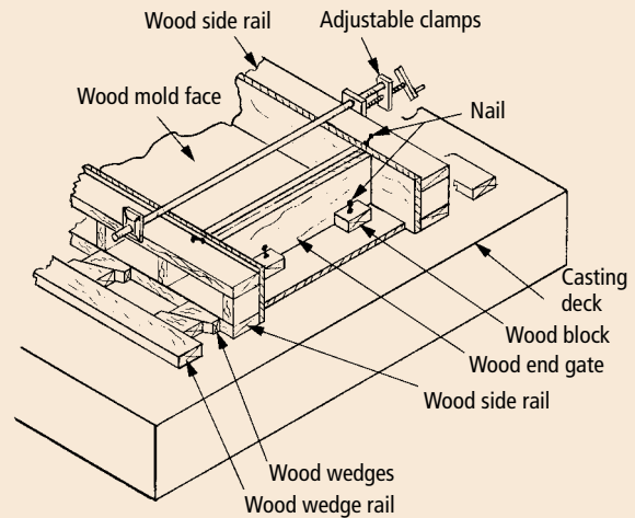
Fig. 2.2.10(b) Removable sections within a mold.
