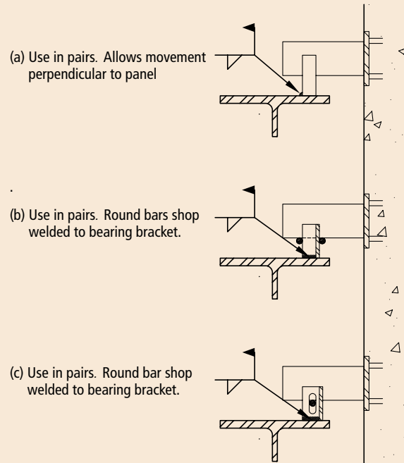
Fig. 4.5.67 Special conditions (SC4). Special shear plates that allow lift-off for rocking
