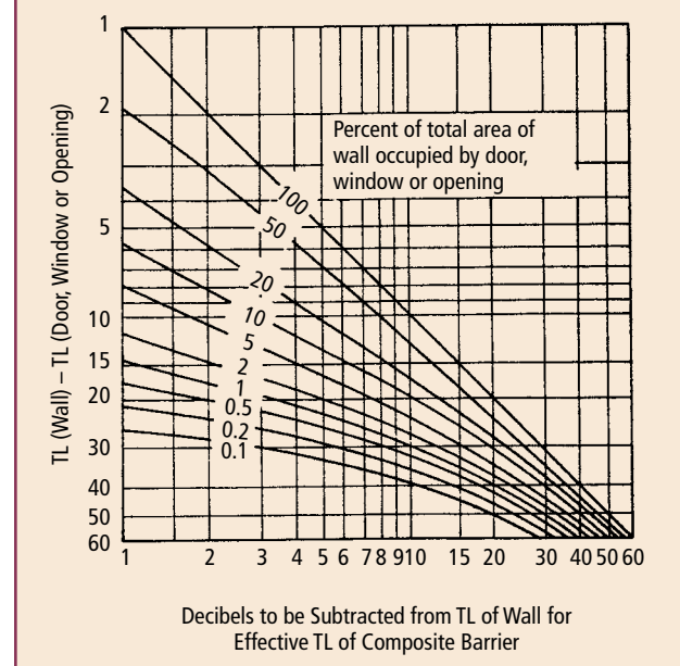
Fig. 5.5.8 Chart for calculating the effective transmission loss of a composite barrier.
