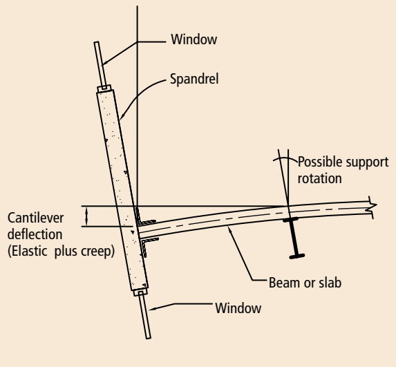
Fig. 4.2.7 Effect of cantilever supports.
