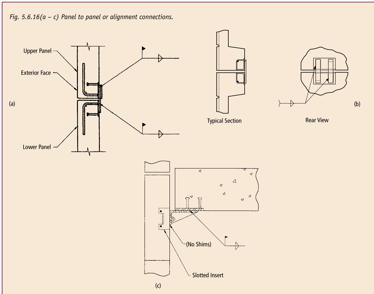
Fig. 5.6.16 – 19 Connection details.
