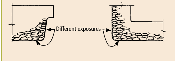
Fig. 3.3.42 Exposure variances caused by aggregate.
