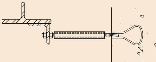
(c) Small diameter tieback rods desired for flexing can be prevented from buckling in compression with loose pipe sleeve
