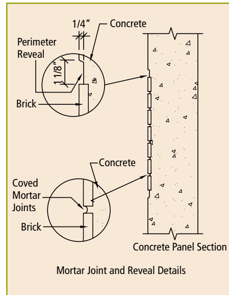
Fig. 3.5.69 Mortar joint and reveal details.
