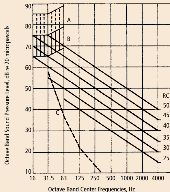
Fig. 5.5.5 Room criteria (RC) curves.
