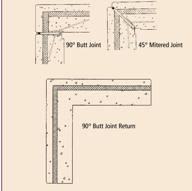
Fig. 5.3.44 Corner variations of sandwich panels.
