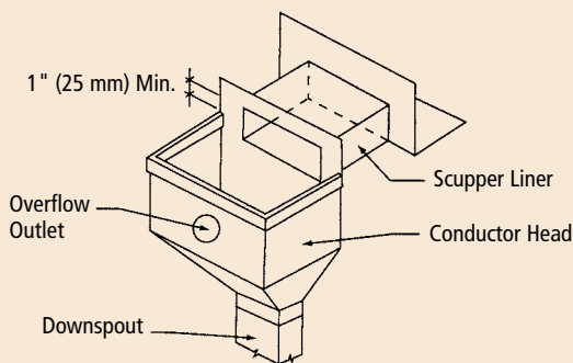
Fig. 5.8.8 Through-wall scupper with conductor head.
