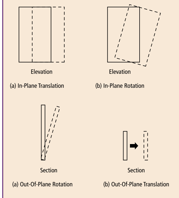
Fig. 4.5.4 Modes of panel response to displacement.
