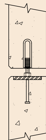
Fig. 4.5.16 Direct bearing (DB2).
