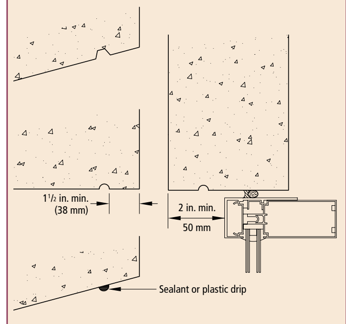
Fig. 5.2.4 Design of water drip in relation to slope.
