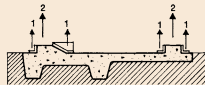
Fig. 2.2.10(a) An envelope mold with haunches on back.
