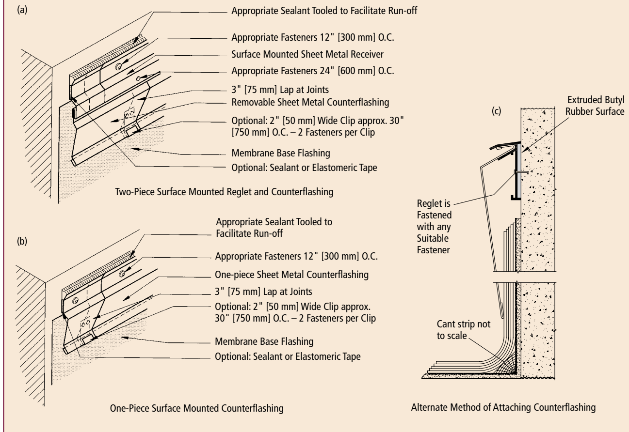
Fig. 5.8.2(a - c) Typical roof flashing details.
