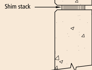
Fig. 4.5.16 Direct bearing (DB2).
