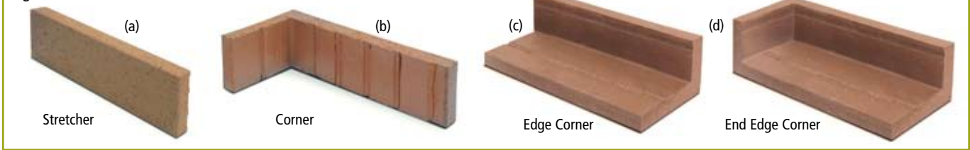
Fig. 3.5.50 Thin brick units.
