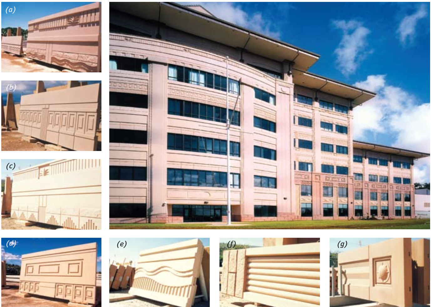
Fig. 3.3.21(a - g) Various patterns integrated into formwork. Nimitz-MacArthur Pacific Command Center, Oahu, Hawaii; Architect: Wimberly Allison Tong & Goo Design; Photos: Gary Hofheimer Photography.
