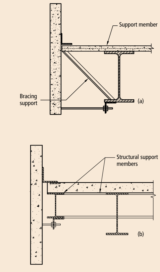
Fig. 4.2.8(a) & (b) Bracing support.
