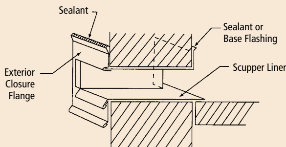
Fig. 5.8.7 Through-wall scupper.
