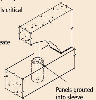
Fig. 4.5.72 Bearing wall to foundation (BWF3).
