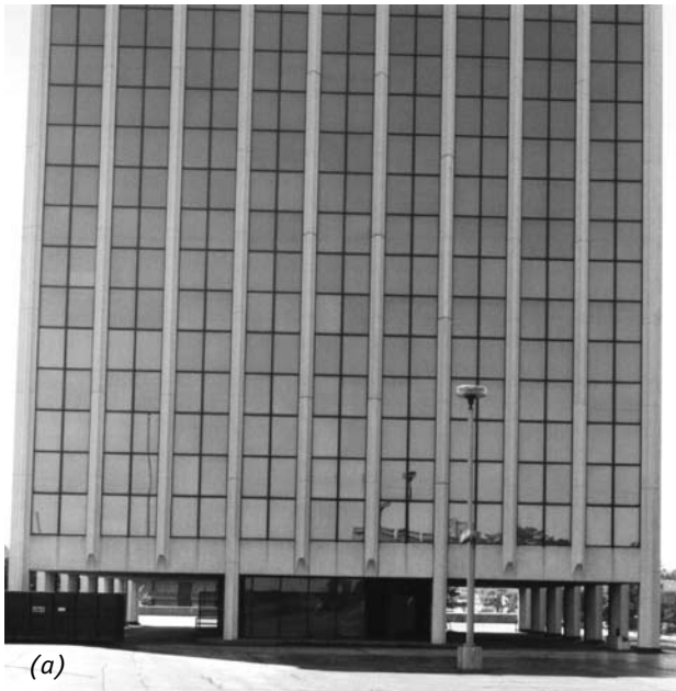
Fig. 5.2.6(a) & (b) Water flow over glass depositing dirt.
