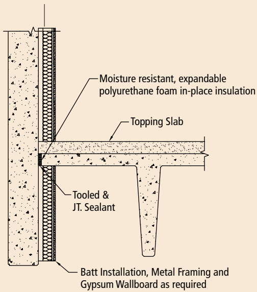
"C" Precast Concrete with Batt Insulation Not to scale
