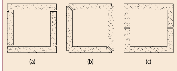
Fig. 5.7.8 Types of column covers.
