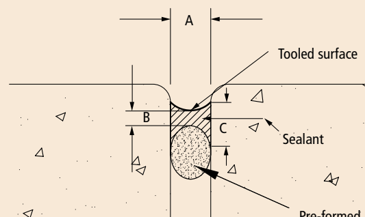
Fig. 4.7.1 Single stage joint.
