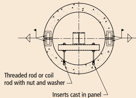
Fig. 4.5.57 Column cover (CC2).
