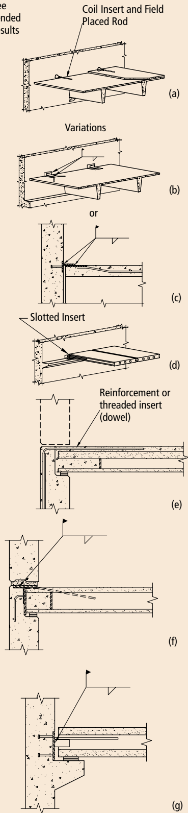
Fig. 4.5.75 Slab to bearing wall (SBW1).
