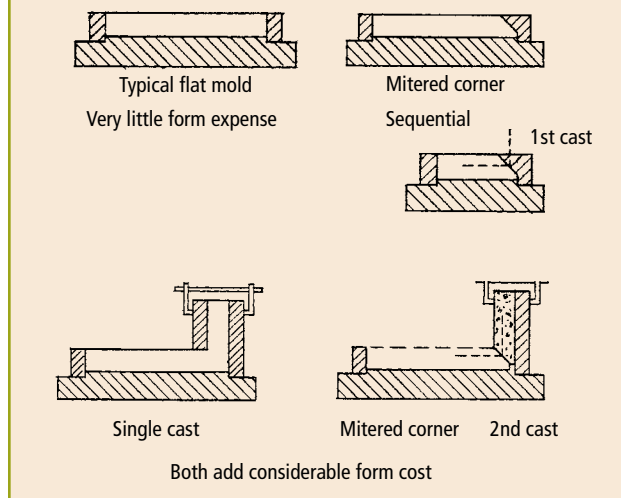
Fig. 3.3.41 Corner – return molds.
