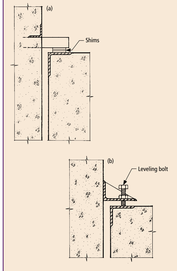
Fig. 4.5.12 Vertical adjustment.
