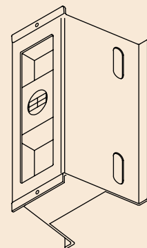
(h) Proprietary threaded embedment. Available with one- or two-way adjustability.
