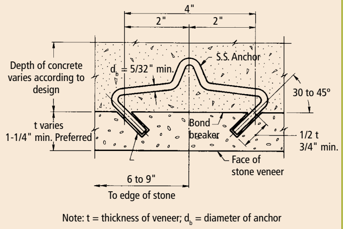
Fig. 3.5.81 Typical anchor for marble veneer.
