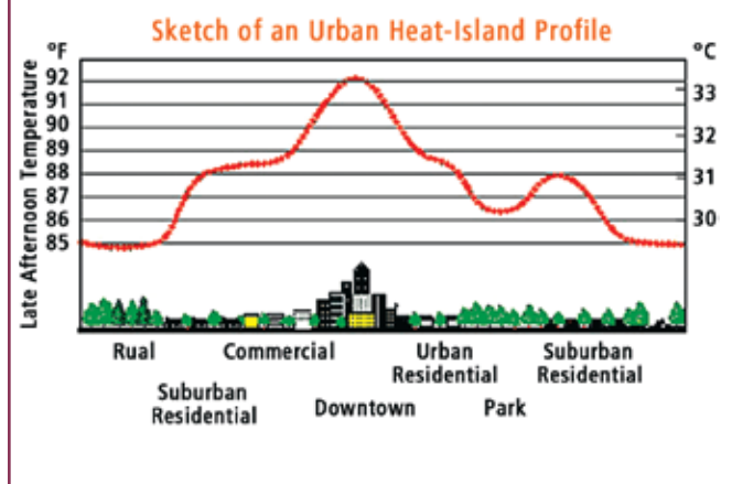
Fig. 5.3.1 Urban heat-island profile (LBNL website).
