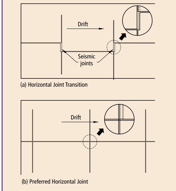
Fig. 4.5.6 Joint elevation changes.
