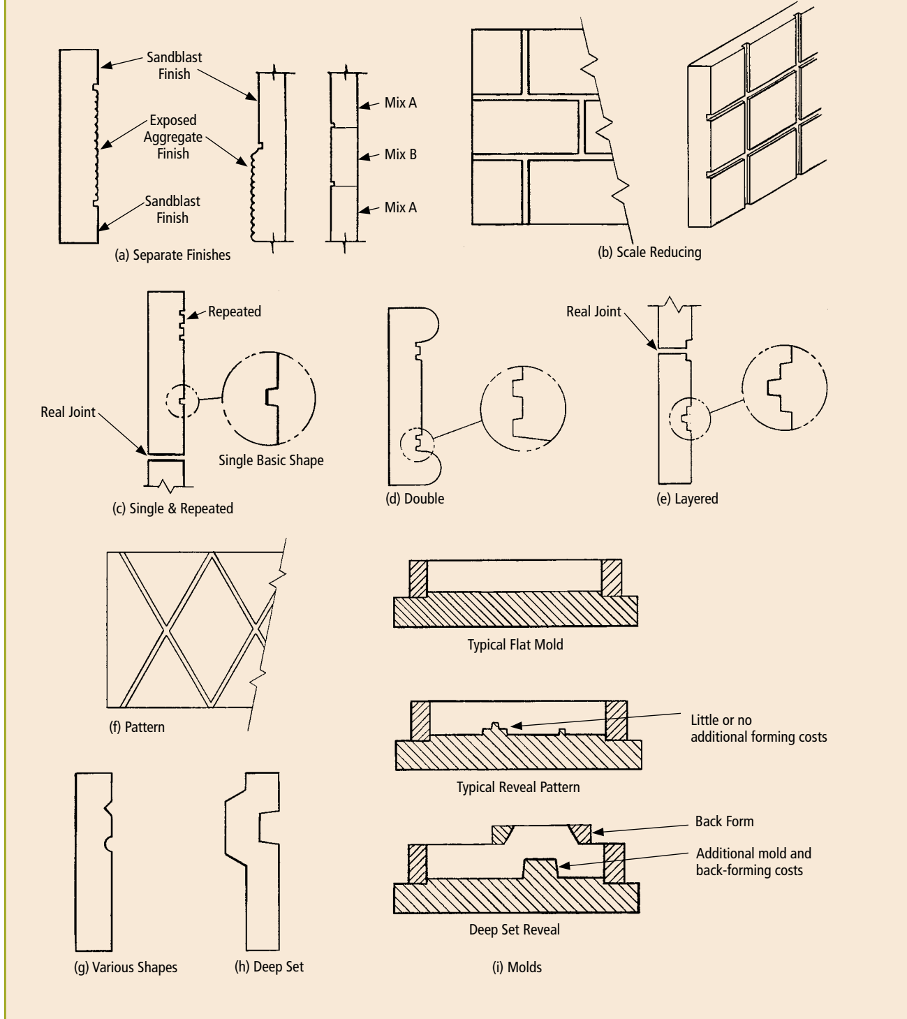
Fig. 3.3.6 Reveals and demarcation features.
