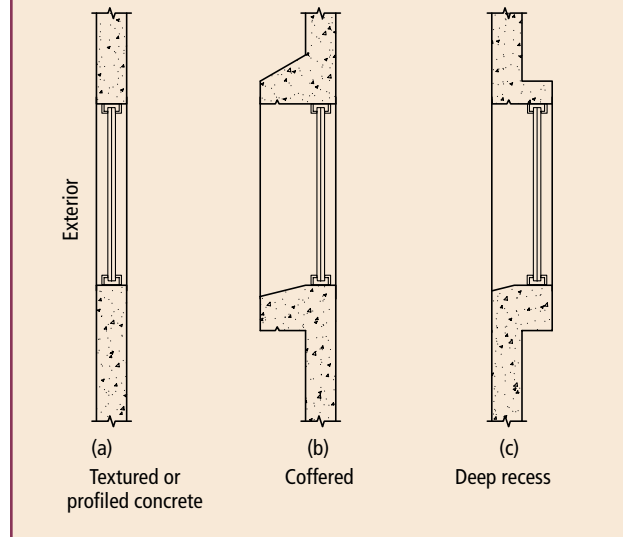
Fig. 5.2.7 Window treatments.
