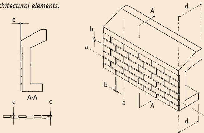
Fig. 3.5.71 Tolerances for brick-faced architectural elements.
