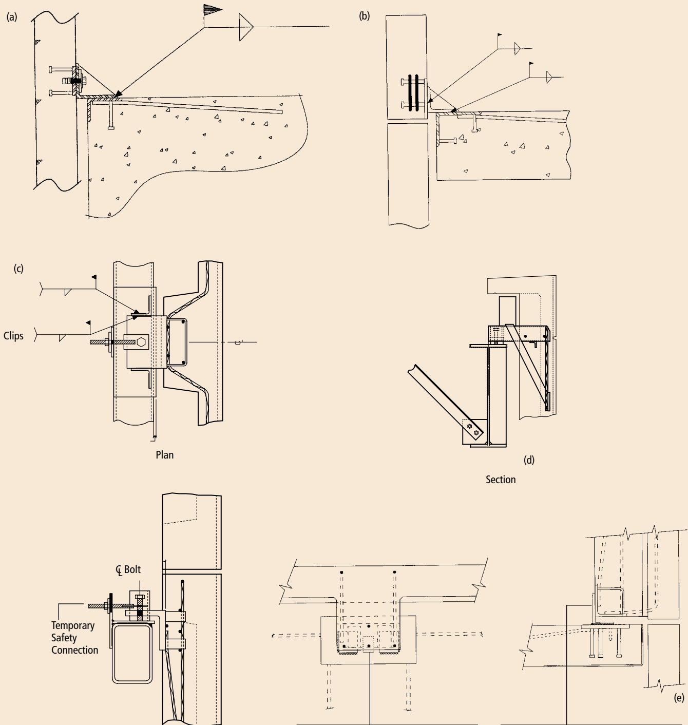
Fig. 5.6.17(a – e) Bearing connections.
