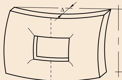
Fig. 4.2.2 Cracking due to restrained bowing.
