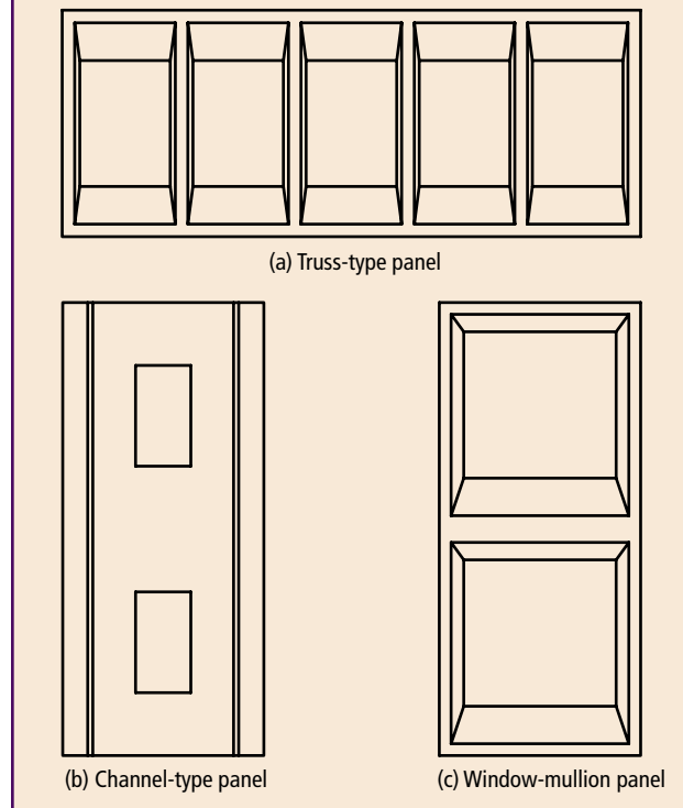
Fig. 4.2.5 Horizontal and vertical rib panels.
