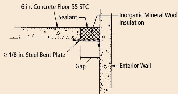
Fig. 5.5.9 Effect of safining insulation seals.
