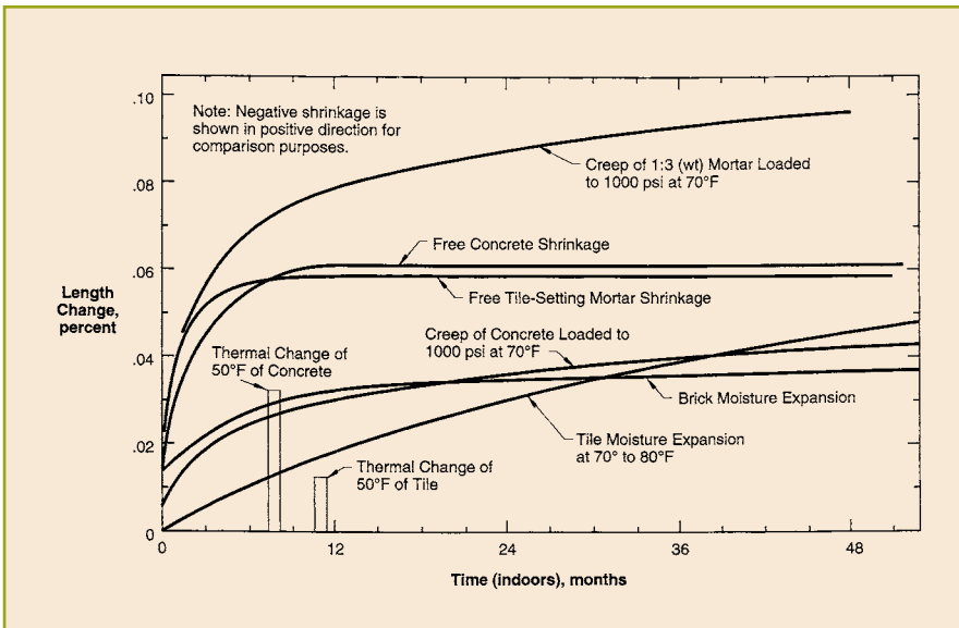
Fig. 3.5.67 Relative temperature and moisture movements of concrete, brick, tile and mortar.
