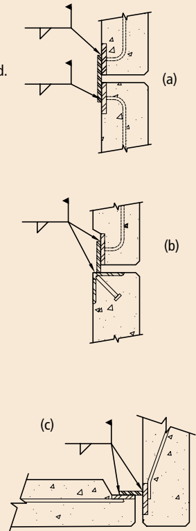
Fig. 4.5.51 Shear plate (SP7).
