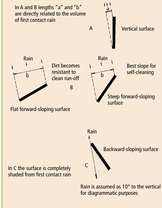
Fig. 3.6.6 Volume of rain likely to hit wall surfaces.
