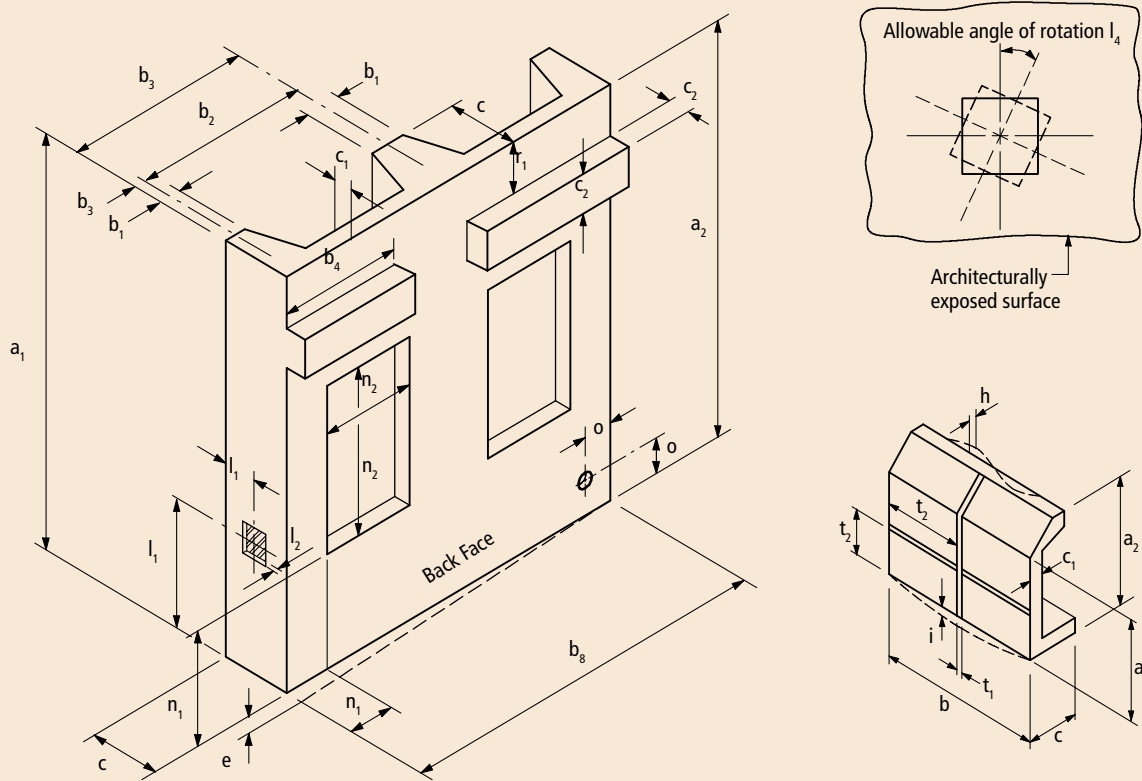
Fig. 4.6.4 Architectural Wall Panels.
