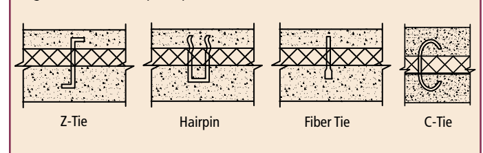
Fig. 5.3.43 Tension/compression ties.
