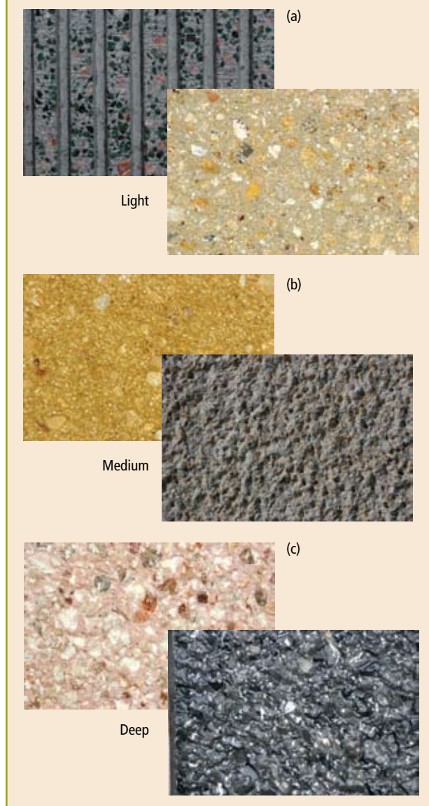
Fig. 3.5.39(a), (b) & (c) Depths of exposure.
