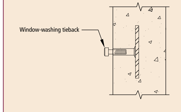
Fig. 5.2.11 Tieback.
