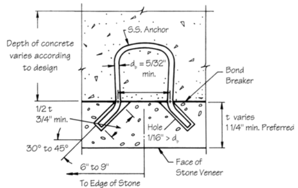
Figure 4 Typical anchor for granite veneer.
