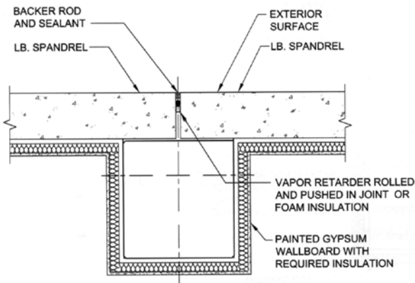
C PRECAST CONCRETE WITH BATT INSULATION NTS
