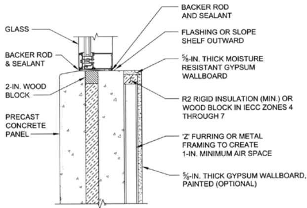
A PRECAST SANDWICH PANEL WALL NTS
