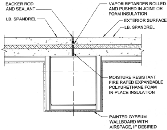
A PRECAST SANDWICH PANEL WALL NTS
