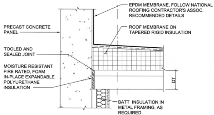
C PRECAST CONCRETE WITH BATT INSULATION NTS
