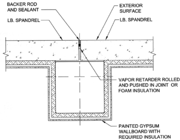
B PRECAST CONCRETE WITH RIGID INSULATION NTS
