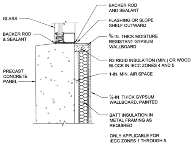
C PRECAST CONCRETE WITH BATT INSULATION NTS
