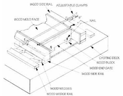
Figure 1E Removable sections within a master mold.
