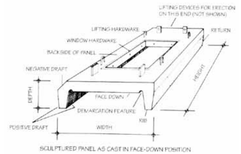
Figure 1D A sculptured panel as cast in a face-down position.
