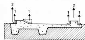
Figure 1F An envelope mold with haunches on the back.
