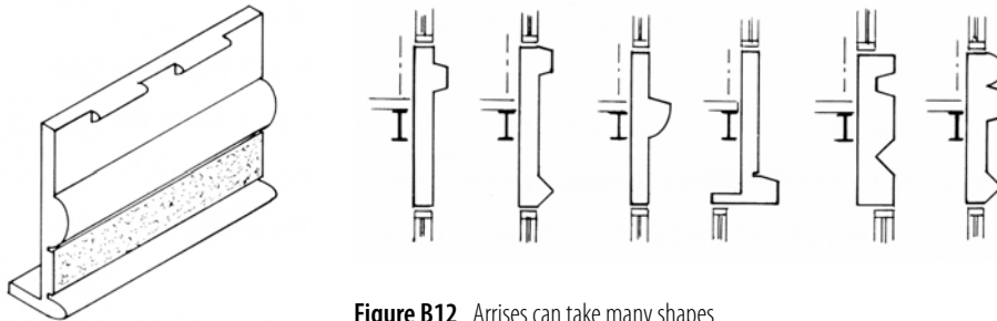
Figure B12 Arrises can take many shapes.
