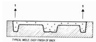
Figure 1G Economy is achieved if the panel can be removed from the mold without disassembling the mold.
