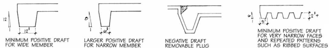
Figure 1H Draft should be increased from 1:12 to 1:6 for panels with special needs.
