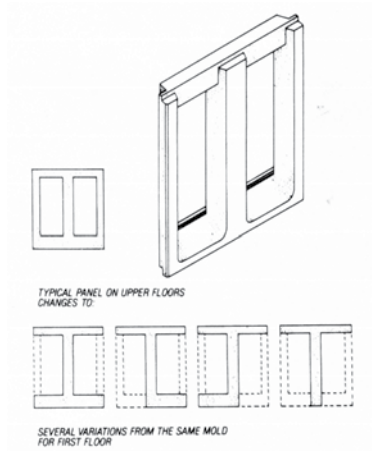
Figure 1A Typical applications of the master mold concept.
