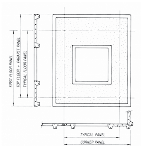
Figure 1C Three views of a master mold.
